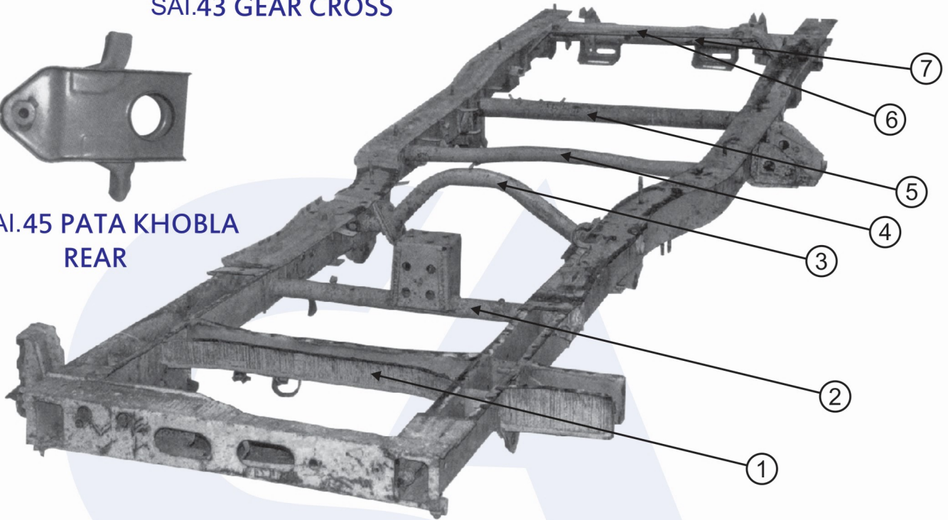
SAI.44 CHASSES FULL ASSY
